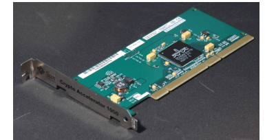
Sun cryptographic accelerator card with integrated hardware number generator
