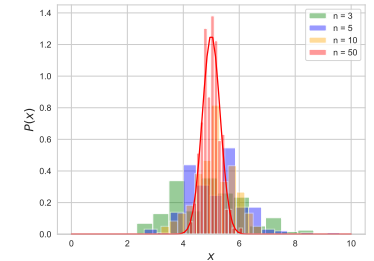
distribution of sample mean for 200 samples of n realisations of X \sim \text{Poiss}(k; 5) and Normal approximation with \text{Norm}(x; 5, \sqrt{\frac{5}{n}})
