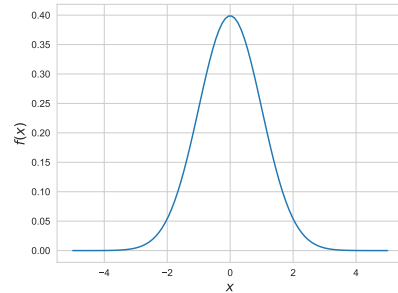
Normal distribution for \mu = 0 and \sigma = 1
