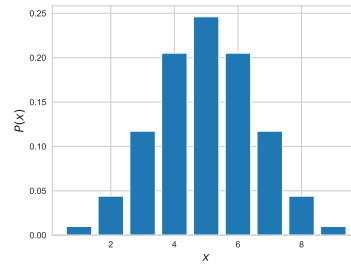
Binomial distribution for n = 10 and p = \frac{1}{2}
