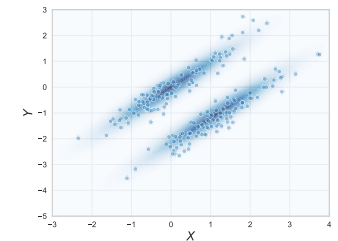
cluster detection based on inference of bivariate Gaussian distributions using Gaussian Mixture Model (GMM)
