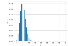
Poisson distribution for \lambda = 5
