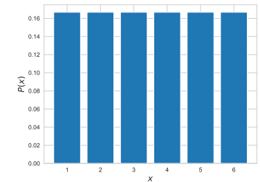
uniform distribution on [1, \dots, 6]
